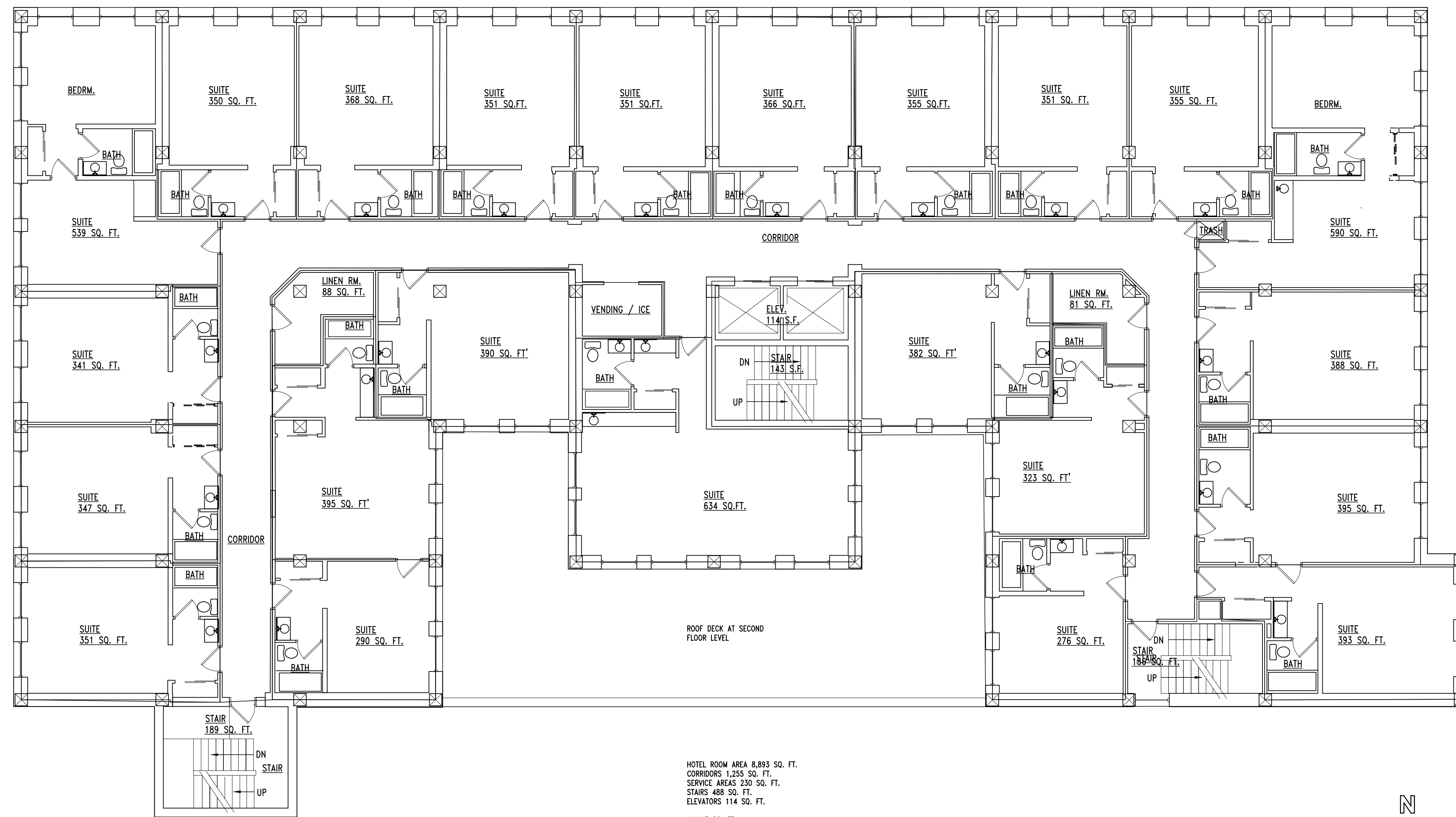
2ND & 3RD FLOOR PLAN 1/8" = 1'-0"
